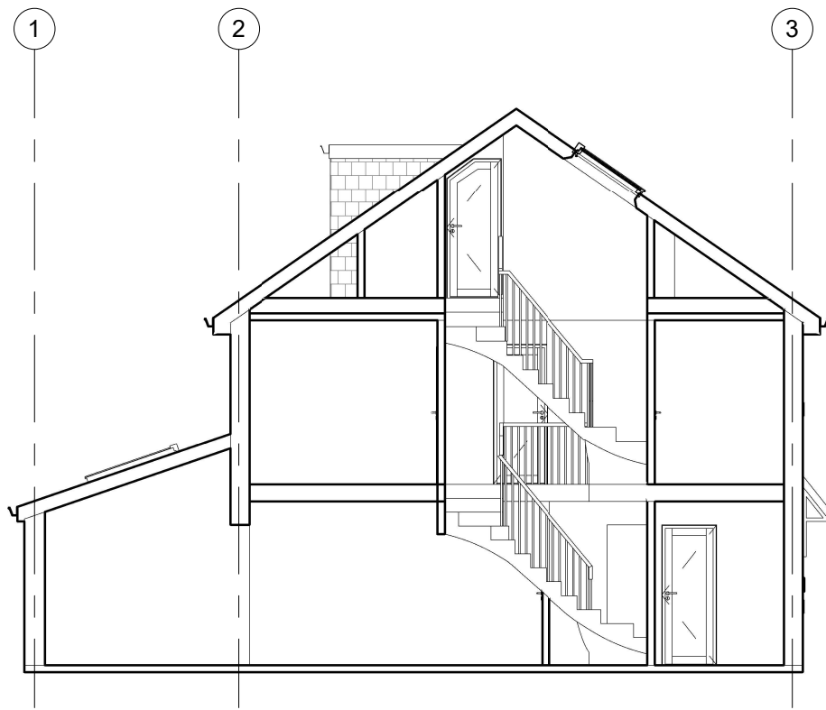
PROPOSED SECTION
