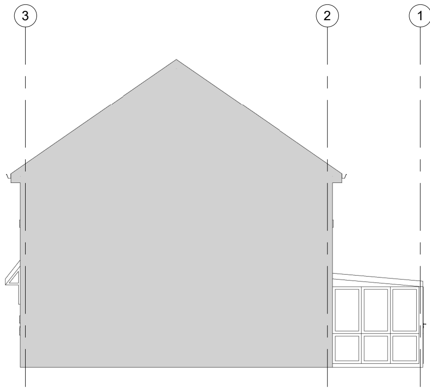
EXISTING RIGHT SIDE ELEVATION
