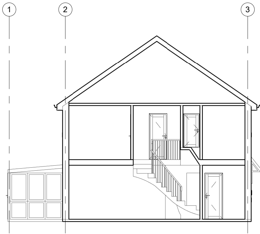
EXISTING SECTION
