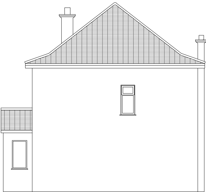
Existing west facing elevation
