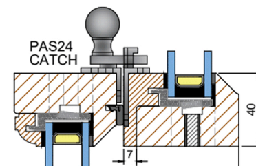
Option sash Horns
