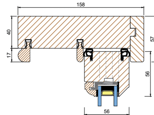
Section B-B - Head and cill
