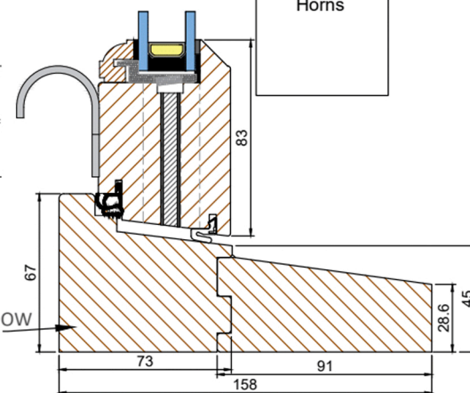
Option sash Horns
