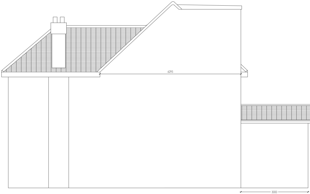
SOUTH ELEVATION
