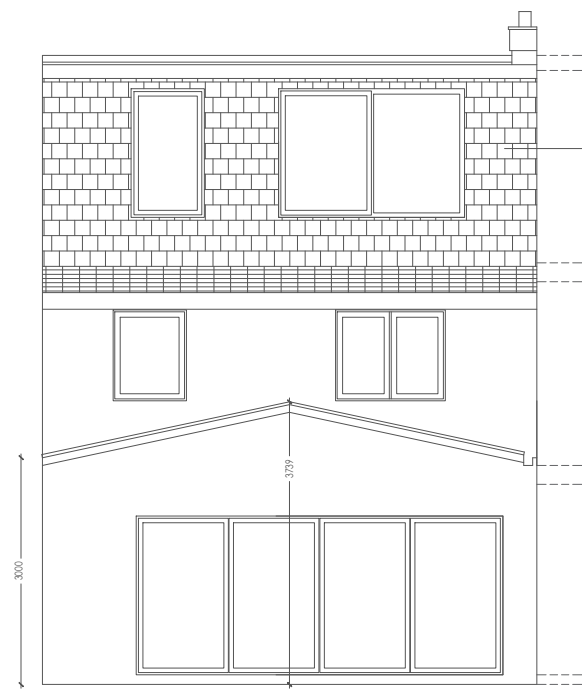
REAR ELEVATION
