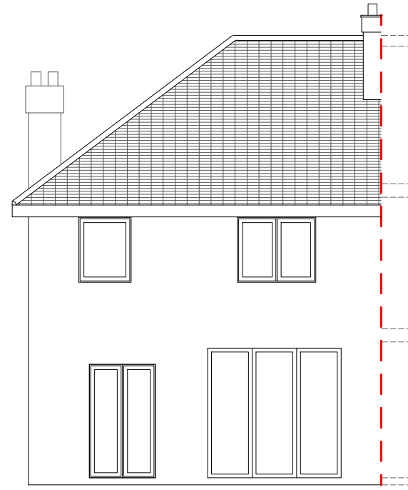
REAR ELEVATION
