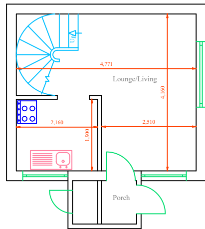
Existing Ground
