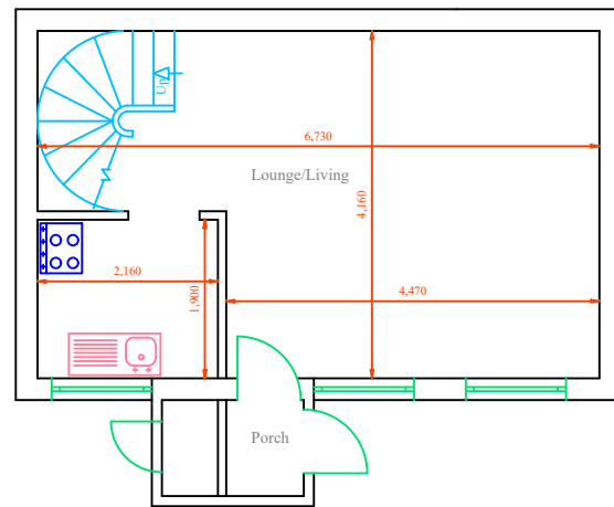
Proposed Ground
