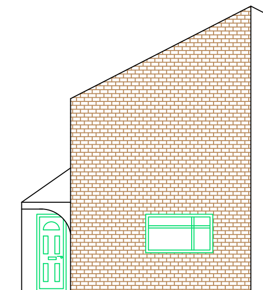
Existing Side Elevation (west)
