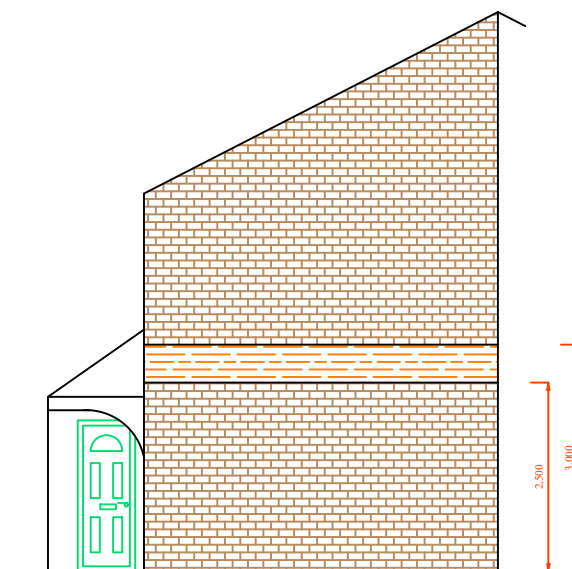
Proposed Side Elevation (west)
