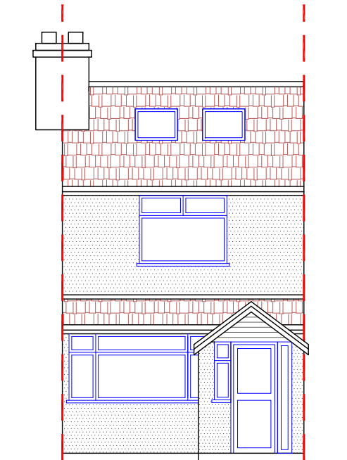
APPROVED FRONT ELEVATION Ref # 76386/APP/2024/1939
