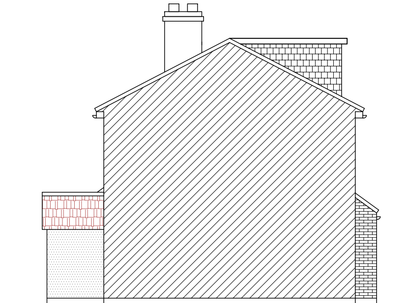
APPROVED SIDE ELEVATION-01 Ref # 76386/APP/2024/1939
