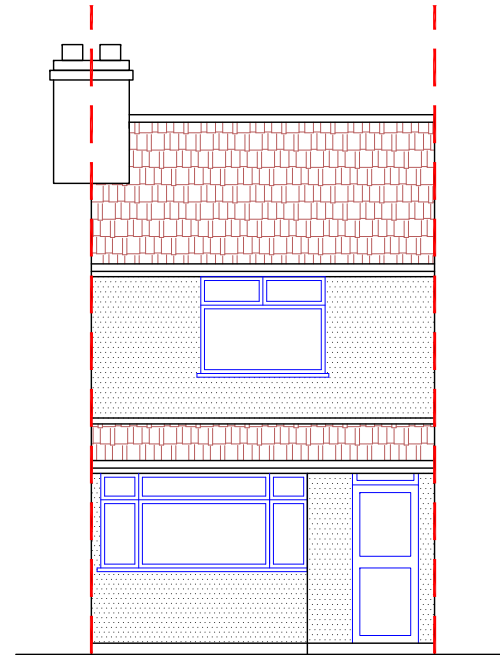
APPROVED FRONT ELEVATION Ref # 76386/APP/2024/1829
