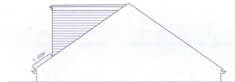
PROPOSED NORTH ELEVATION SCALE 1/100
