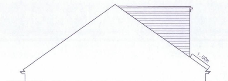
PROPOSED SOUTH ELEVATION SCALE 1/100
