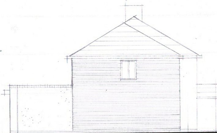
WEST ELEVATION
