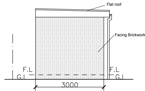
PROPOSED OUTBUILDING SIDE ELEVATION
