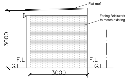
PROPOSED OUTBUILDING SIDE ELEVATION
