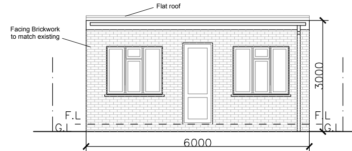
PROPOSED OUTBUILDING FRONT ELEVATION
