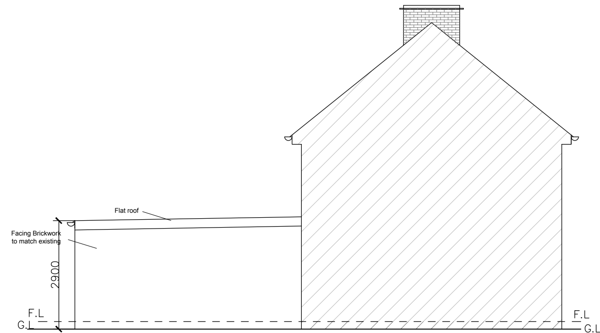
PROPOSED APPROVED SIDE ELEVATION
