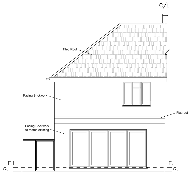
PROPOSED APPROVED REAR ELEVATION
