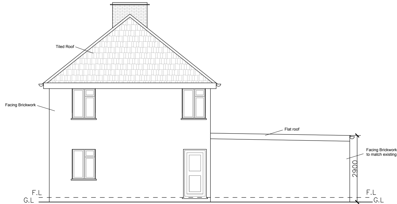
PROPOSED APPROVED SIDE ELEVATION
