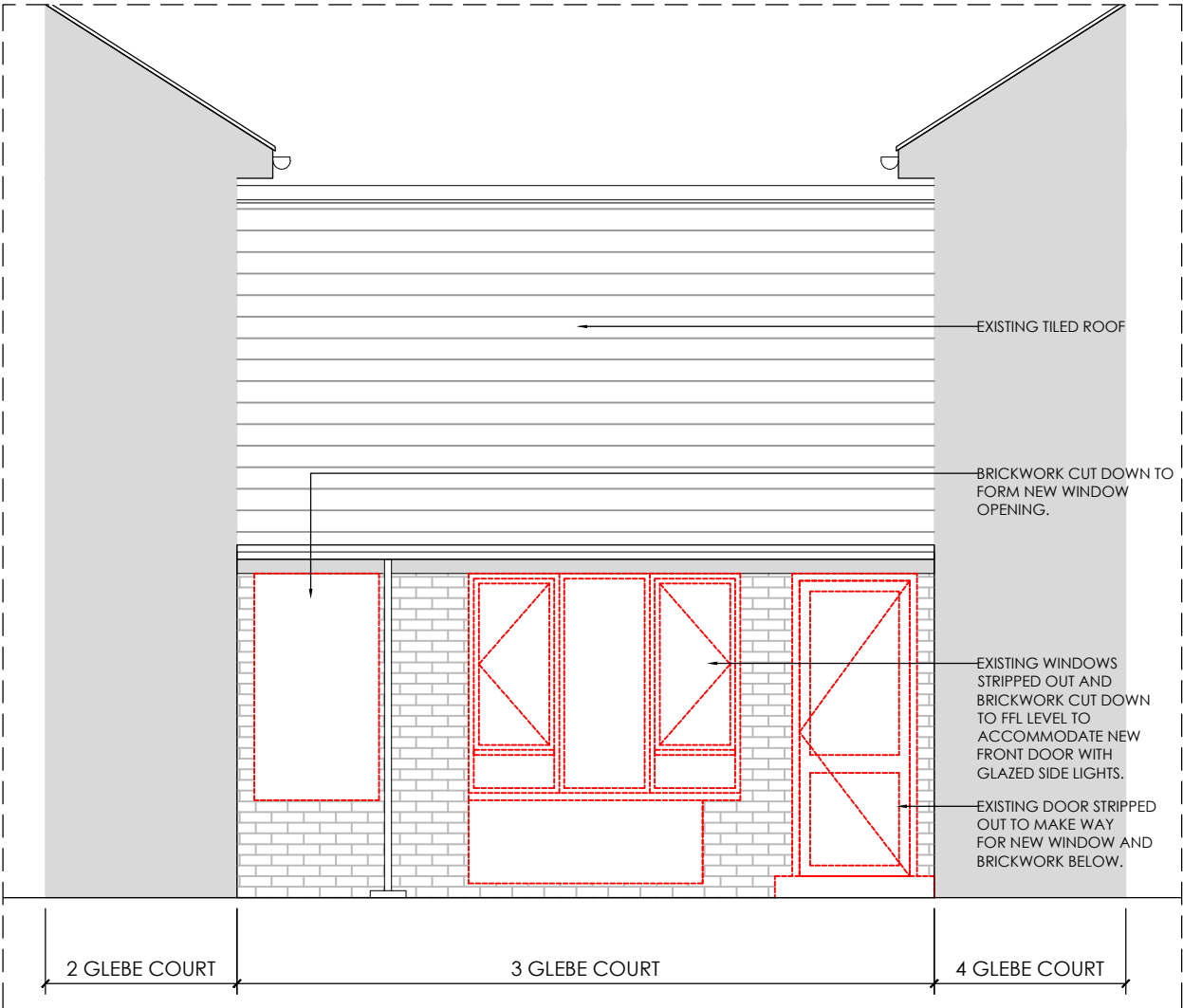
FRONT DEMOLITION ELEVATION
