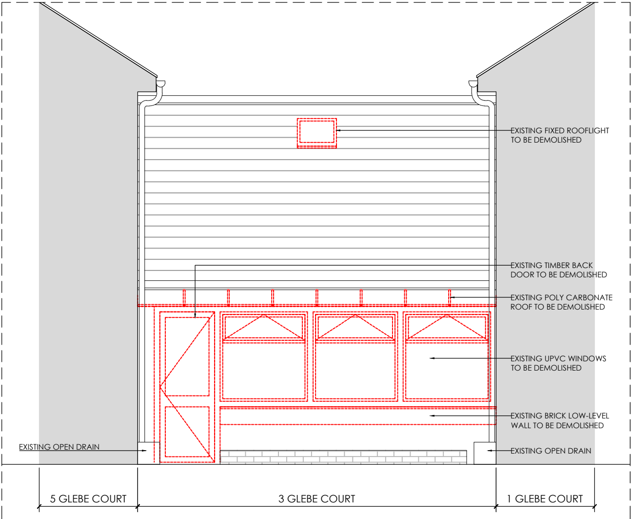
REAR DEMOLITION ELEVATION
