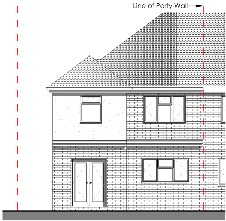
5 Existing Rear Elevation 2549-A-100 1 : 100
