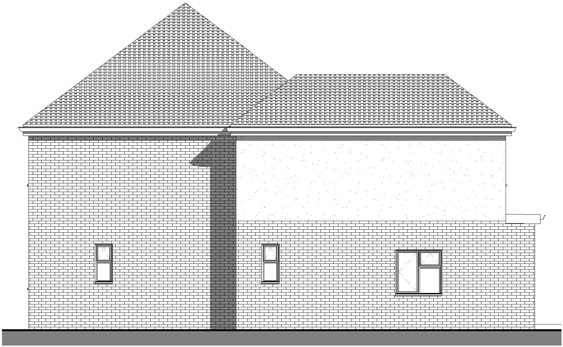
7 Existing Side Elevation 02 2549-A-100 1 : 100
