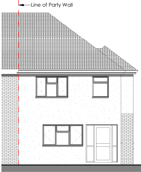
4 Existing Front Elevation 2549-A-100 1 : 100
