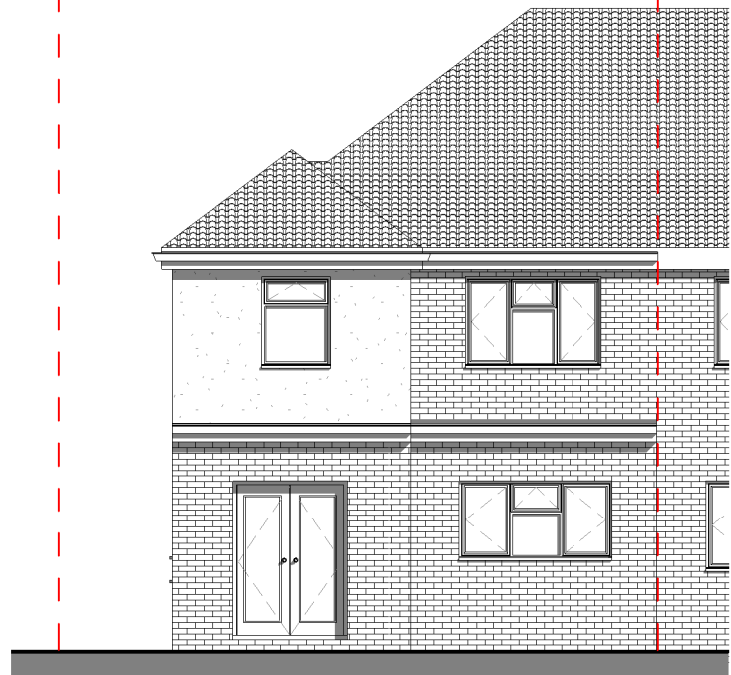
5 Existing Rear Elevation 2549-A-100 1 : 100
