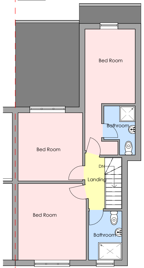
2 Existing First Floor 2549-A-100 1 : 100
