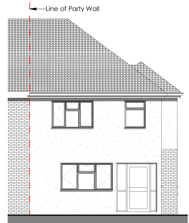
4 Existing Front Elevation 2549-A-100 1 : 100
