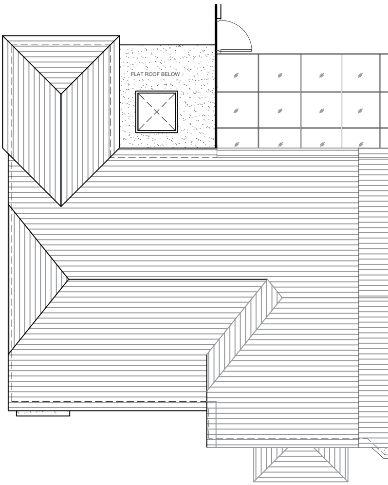
03 - ROOF PLAN
