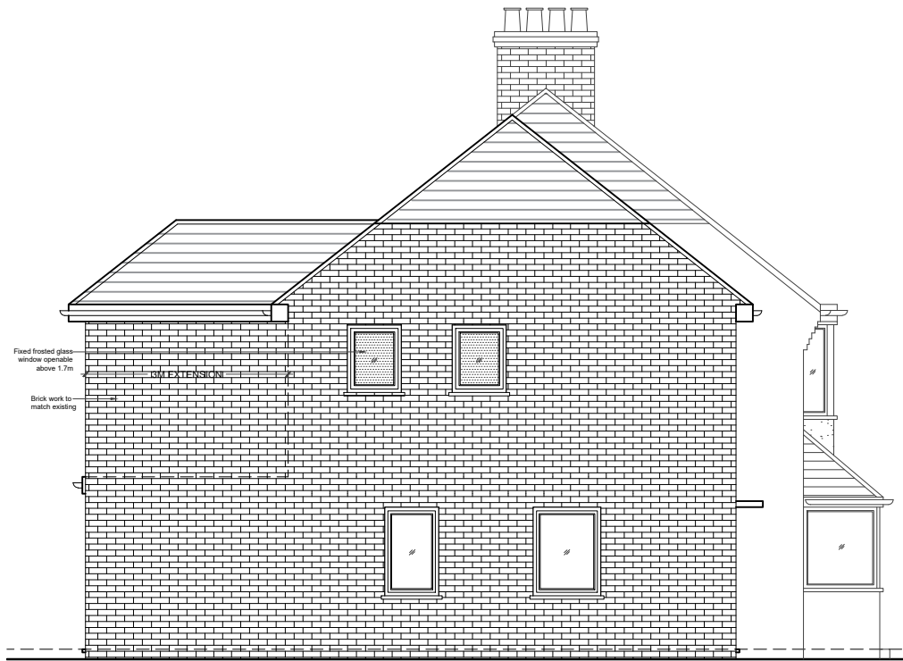
06 - SIDE ELEVATION
