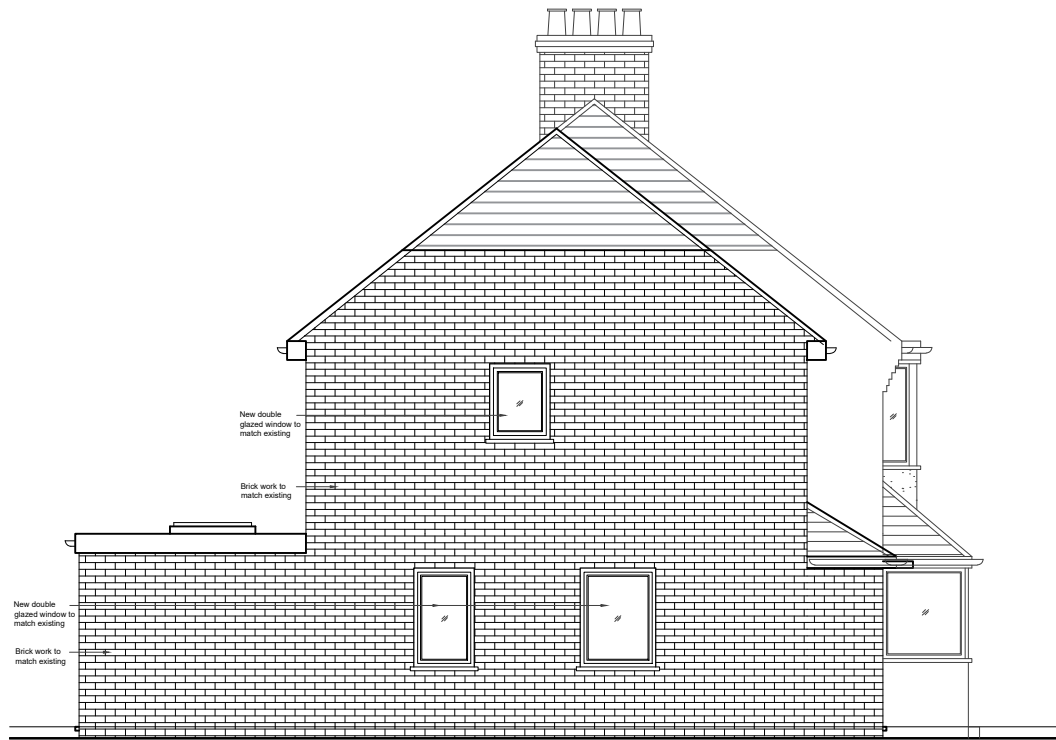
03- SIDE ELEVATION
