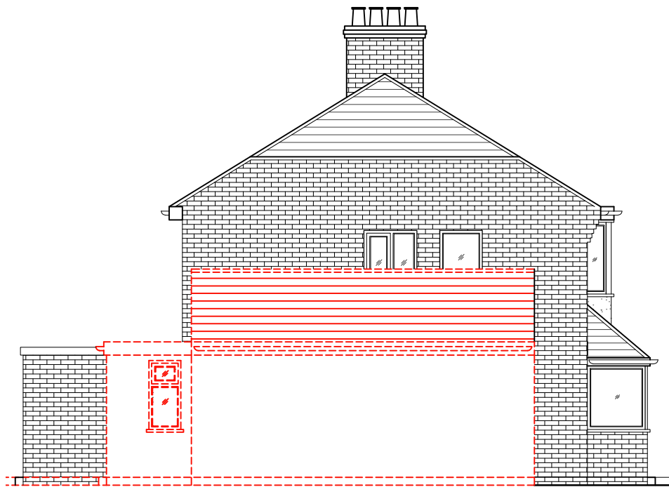
03 - SIDE ELEVATION
