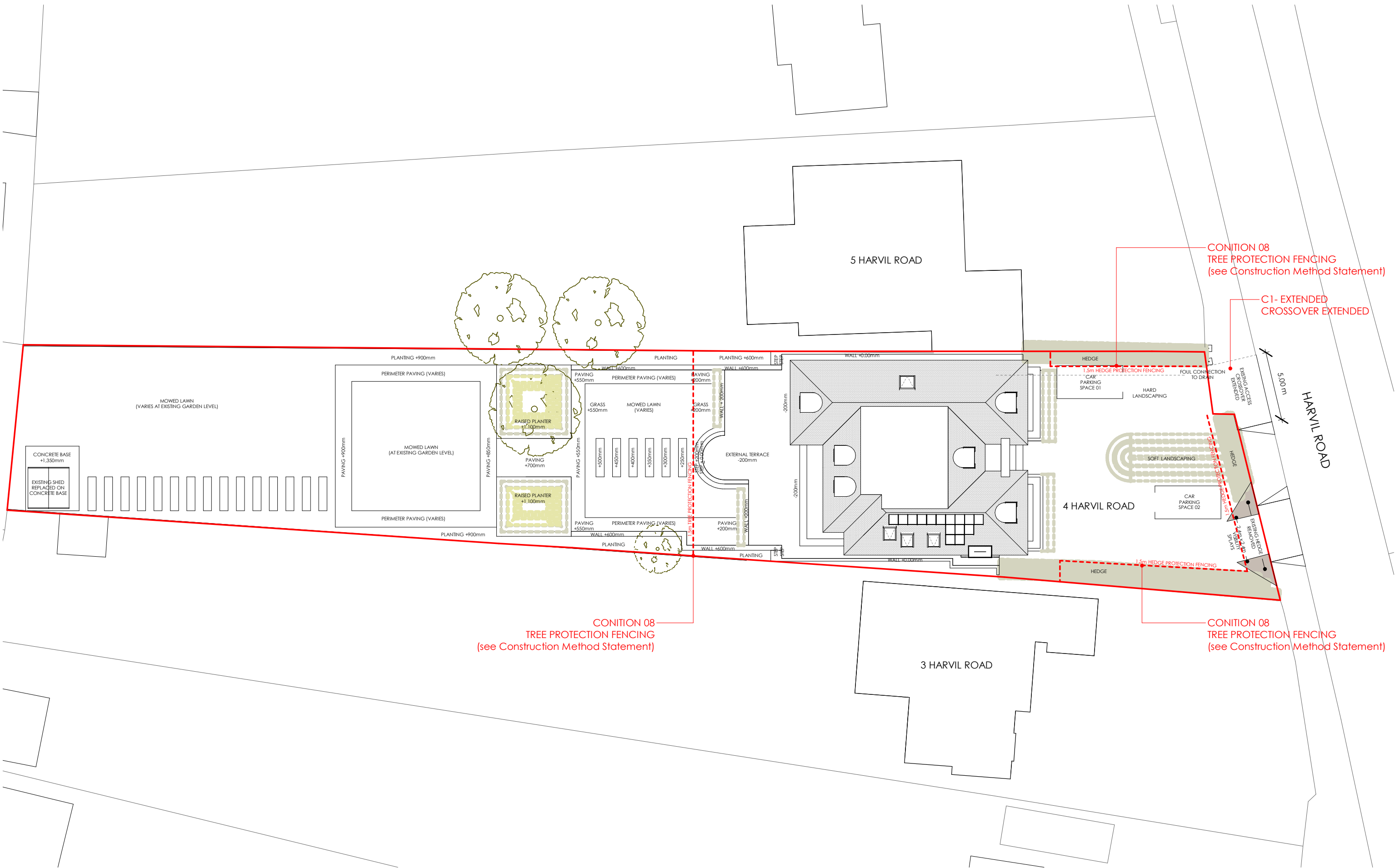
C354-10 Proposed Block Plan (Rev E)
