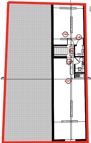
FIRST FLOOR PLAN (EXISTING)
