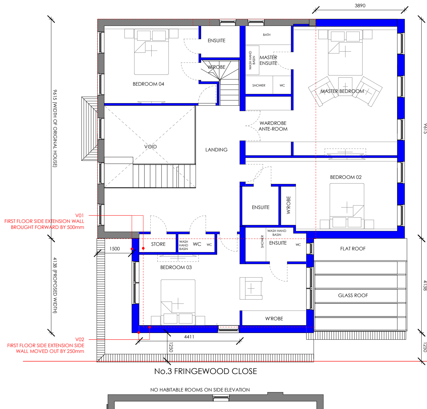
23.01 Proposed First Floor Plan C374 - 23 Proposed First and Loft Floor Plans (Rev D)
