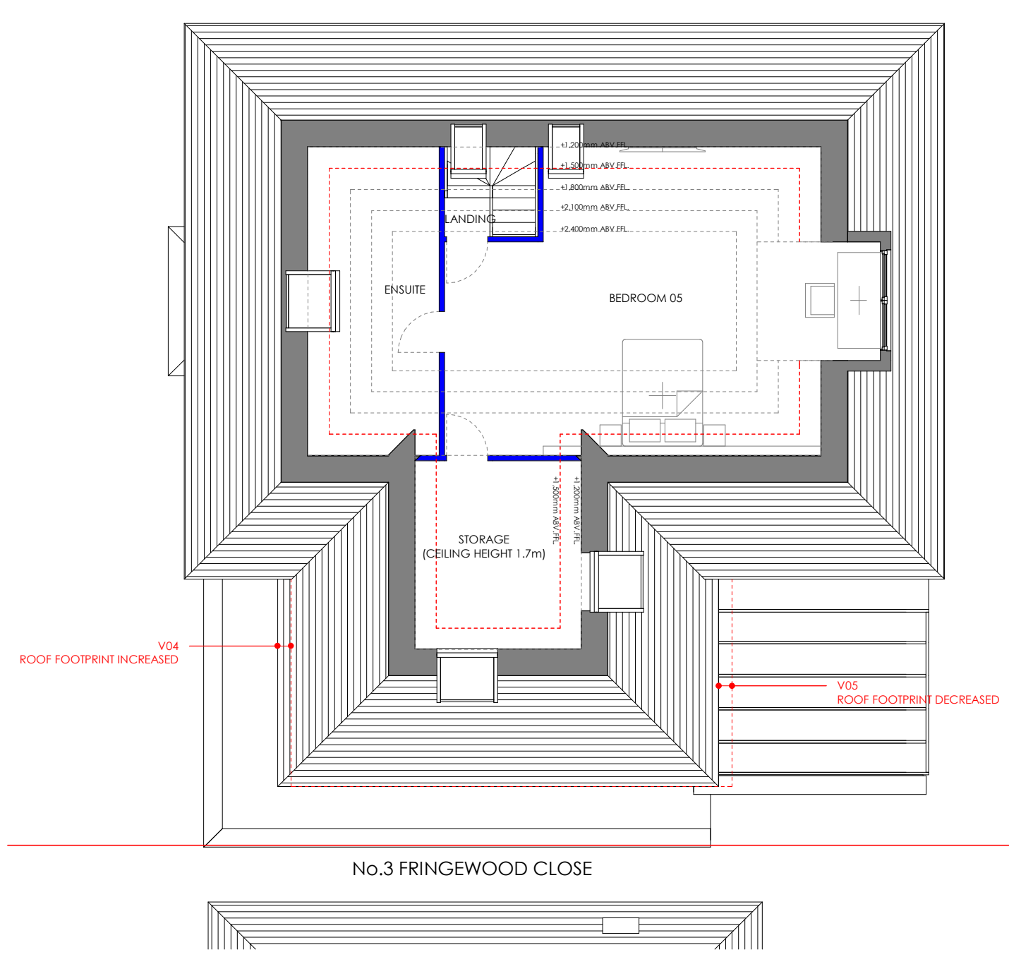
23.02 Proposed Loft Plan
