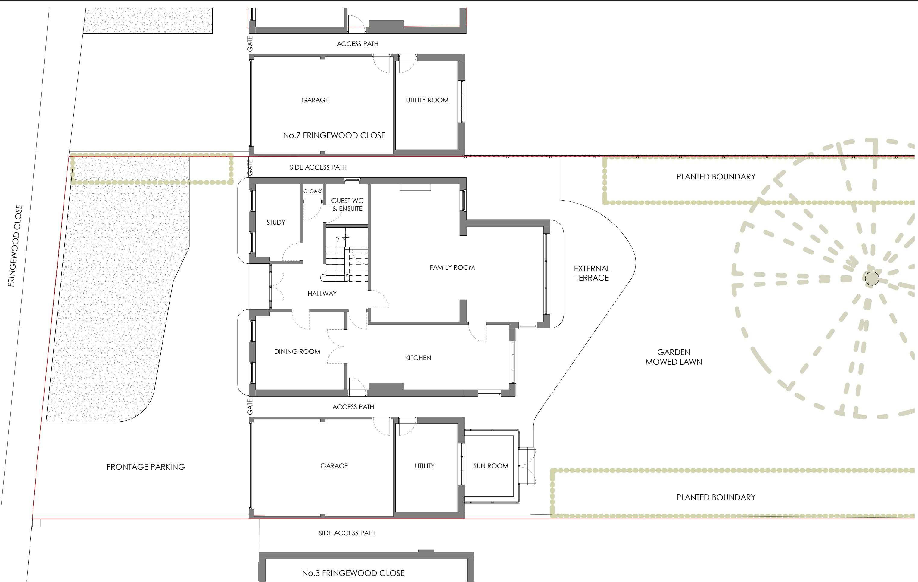
C374 - 12 Existing Ground Floor Plan (Rev D)
