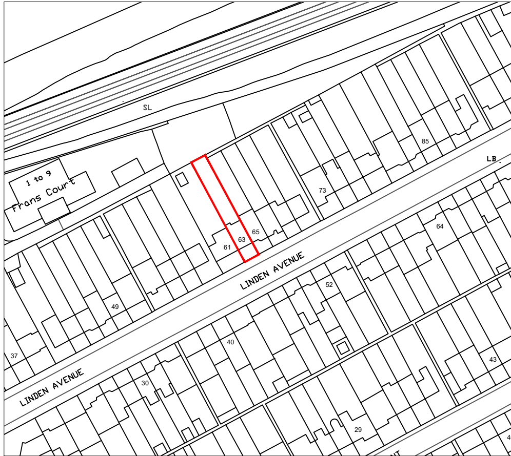
SITE PLAN (1:1250)
