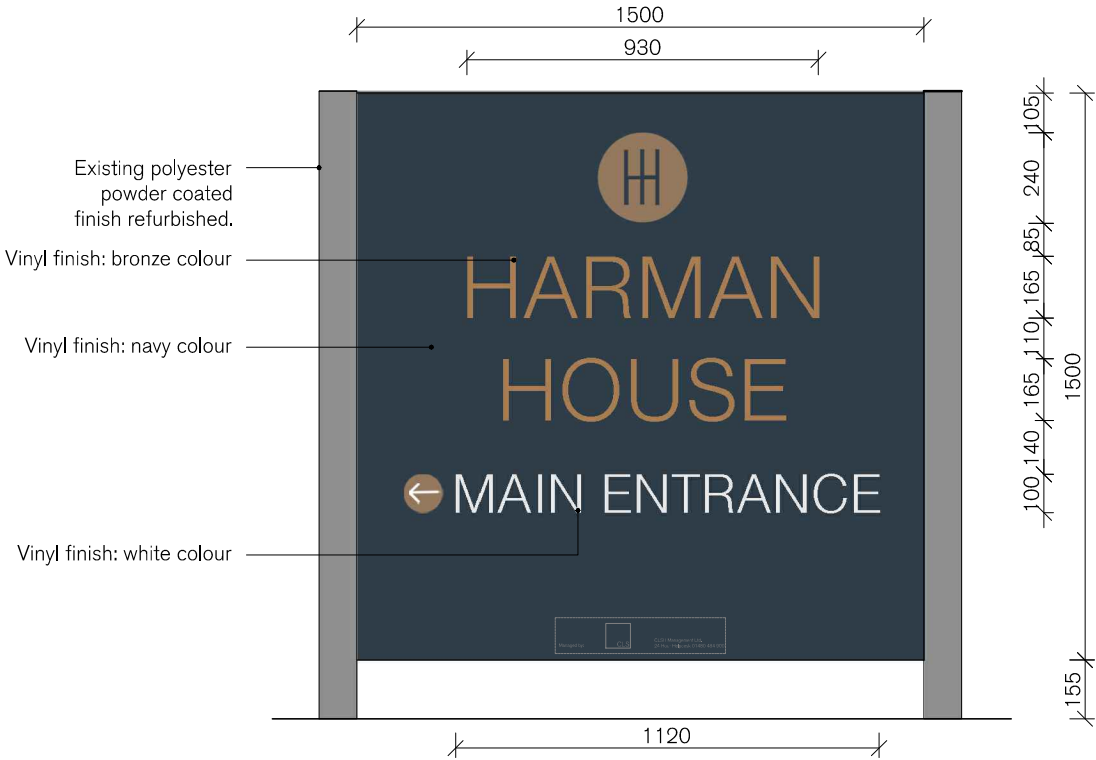
1 Proposed Front Elevation Sign A 1:20
