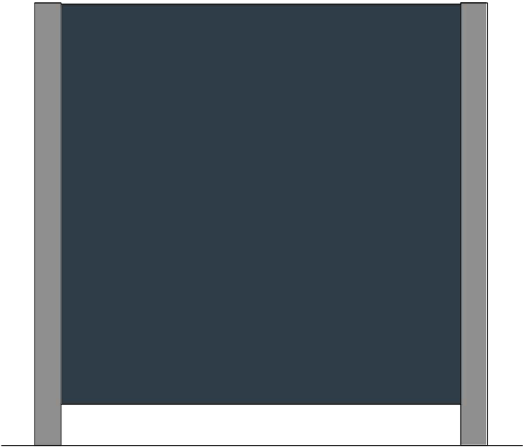
2 Proposed Rear Elevation Sign C 1:20
