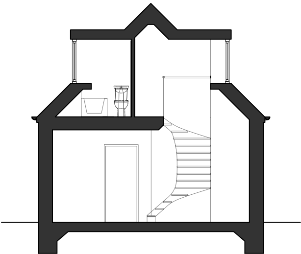
EXISTING SECTION 1:100
