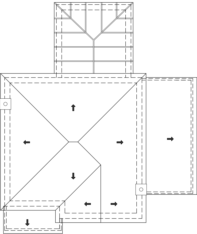
ROOF PLAN Total GIA: 138.8 sqm
