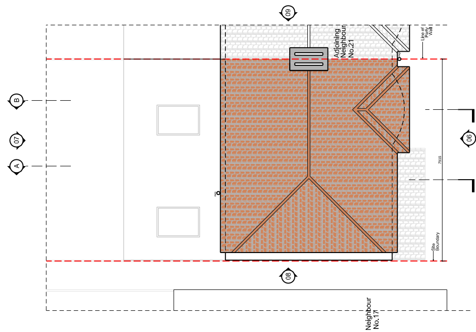
03 ROOF PLAN 1:100
