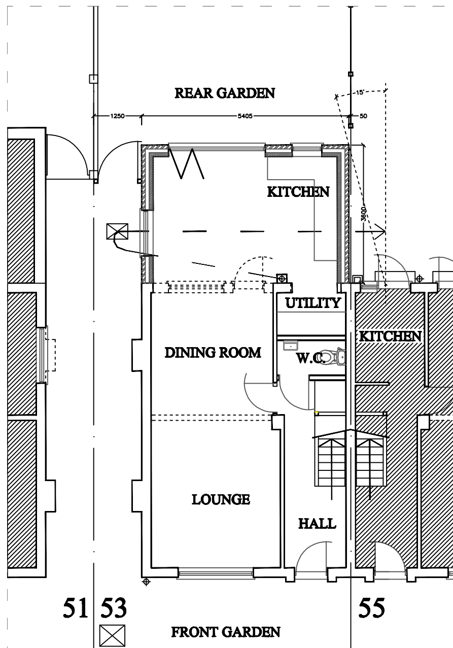
GROUND FLOOR
