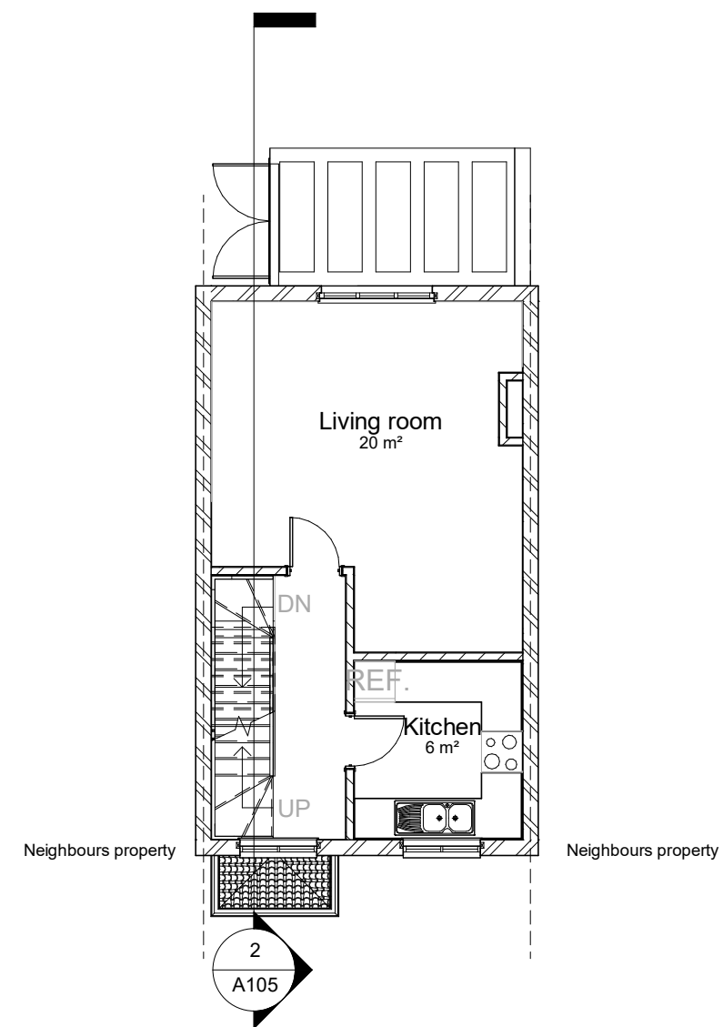
2 01-First floor - Proposed 1 : 100
