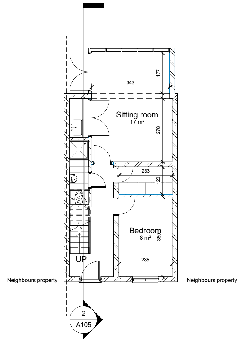
2 00-Ground floor - Proposed 1 : 100
