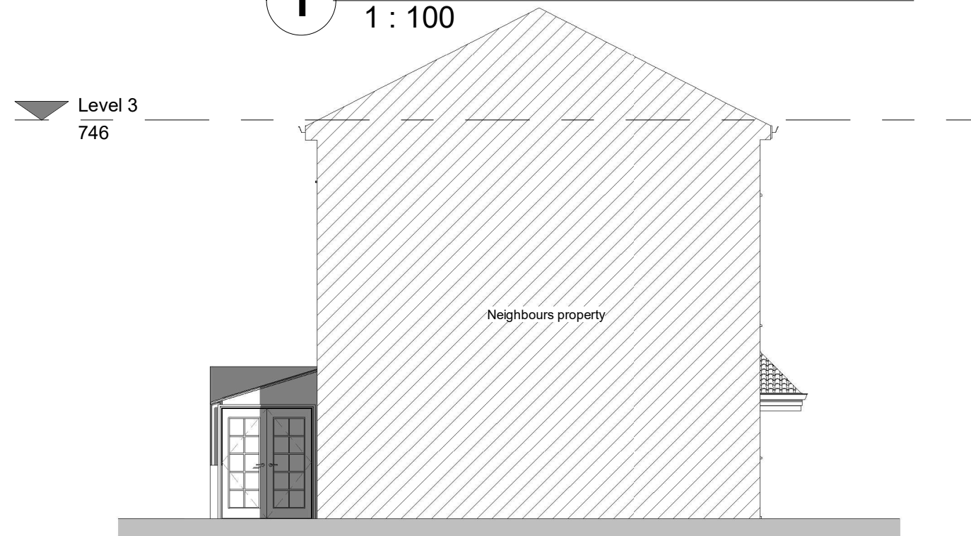
2 West elevation - Proposed 1 : 100
