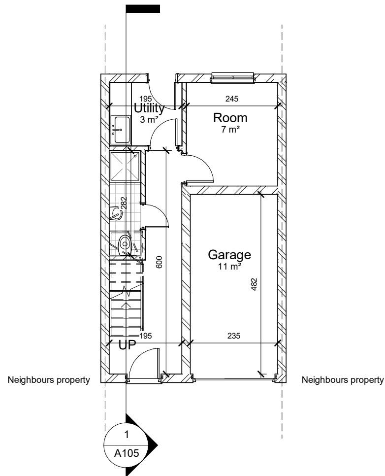
1 00-Ground floor - Existing 1 : 100
