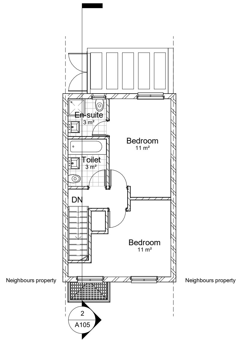
1 02 - Second Floor - Proposed 1 : 100
