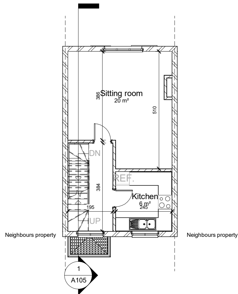
1 01-First floor - Existing 1 : 100
