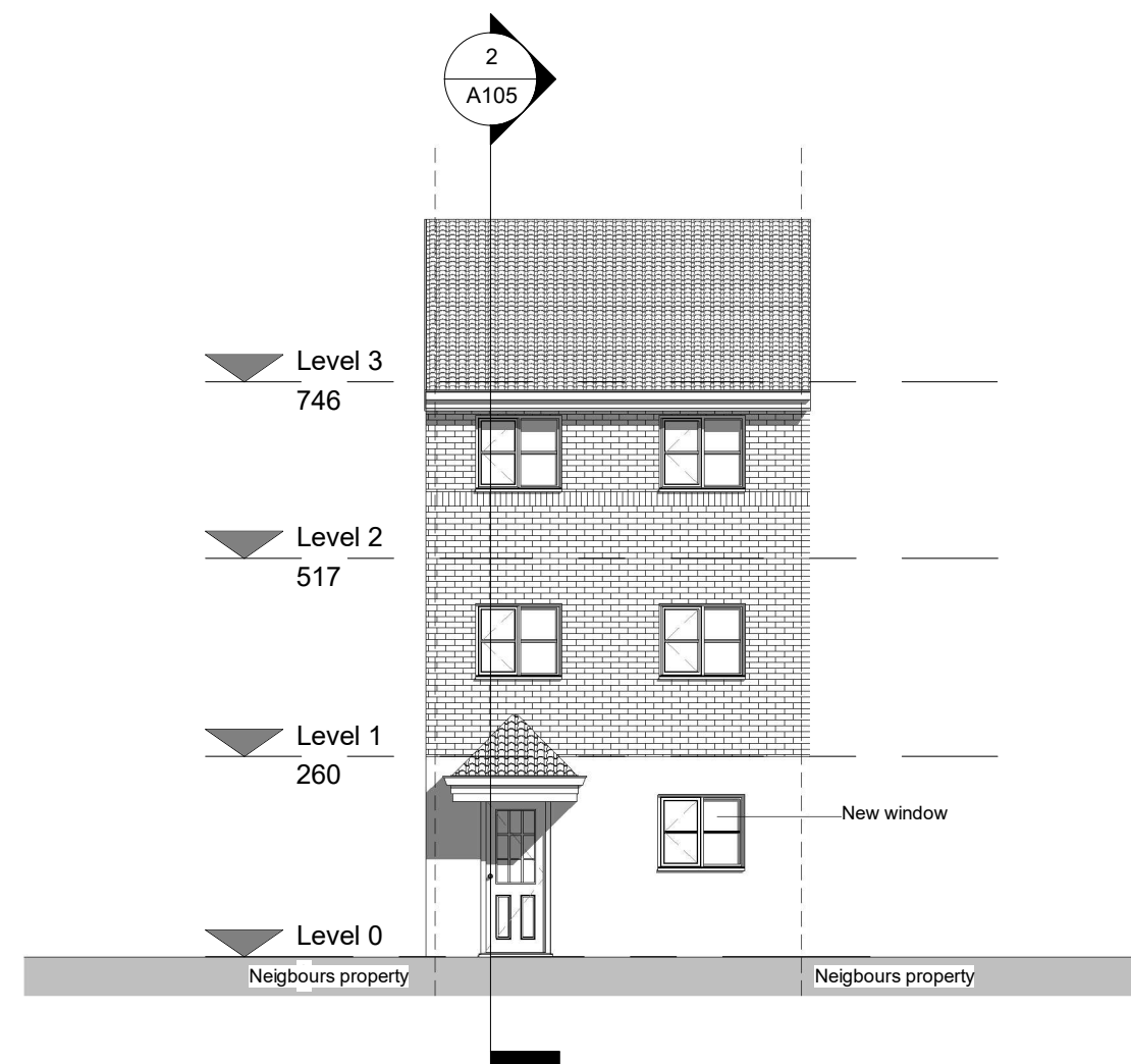
2 Front elevation - Proposed 1 : 100
