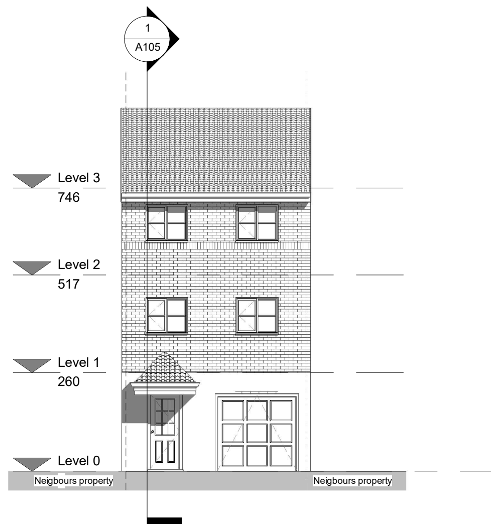
1 Front elevation - Existing 1 : 100
