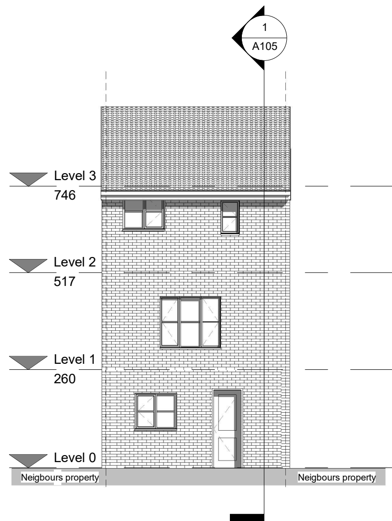
1 Rear elevation - Existing 1 : 100
