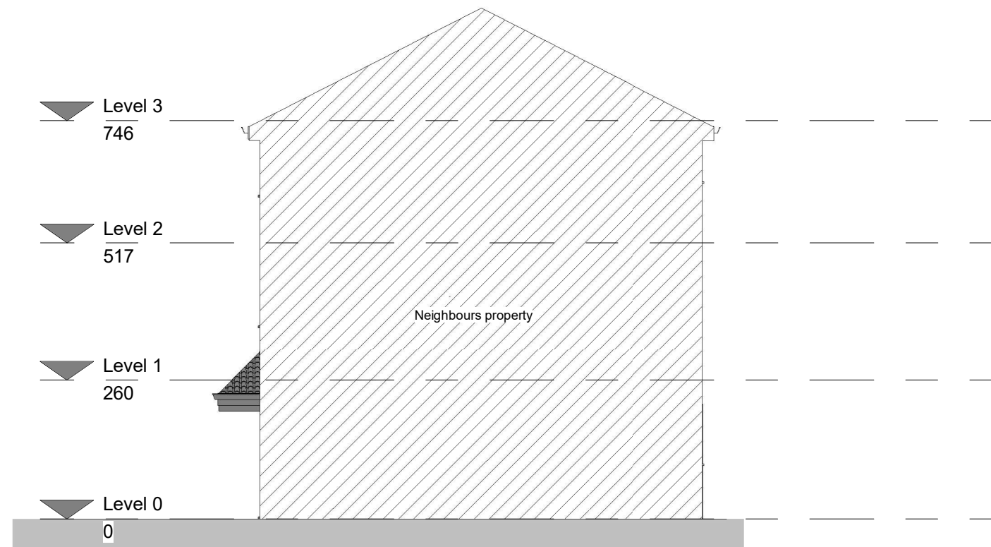
1 East elevation - Existing 1 : 100
