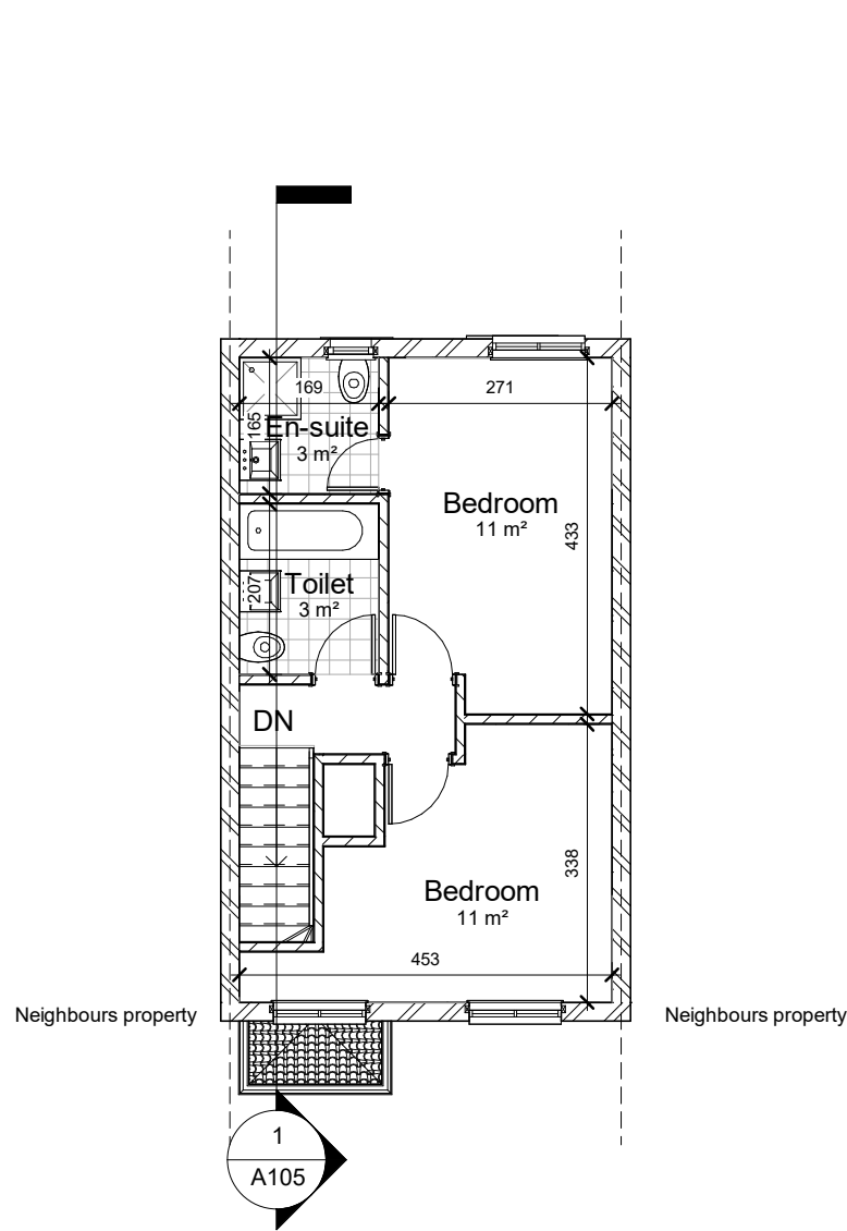
2 02 - Second Floor - Existing 1 : 100
