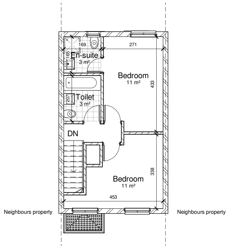
2 02 - Second Floor - Existing 1 : 100
