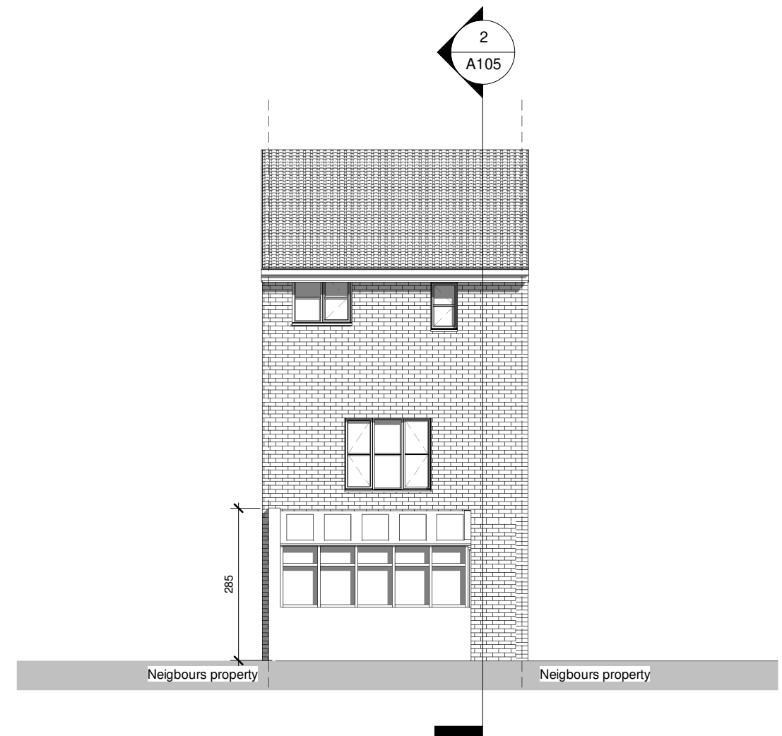
2 Rear elevation - Proposed 1 : 100
