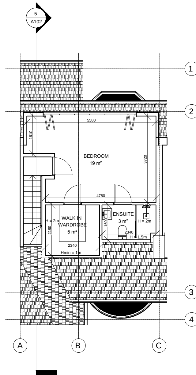
PROPOSED LOFT FLOOR PLAN
