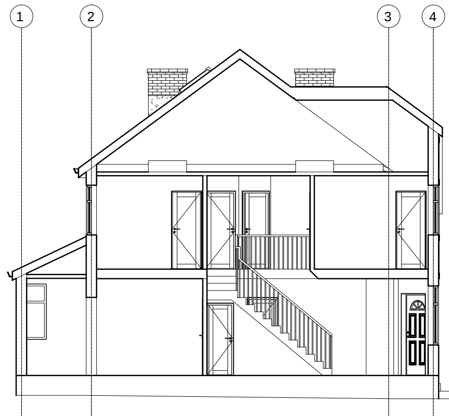
EXISTING SECTION
