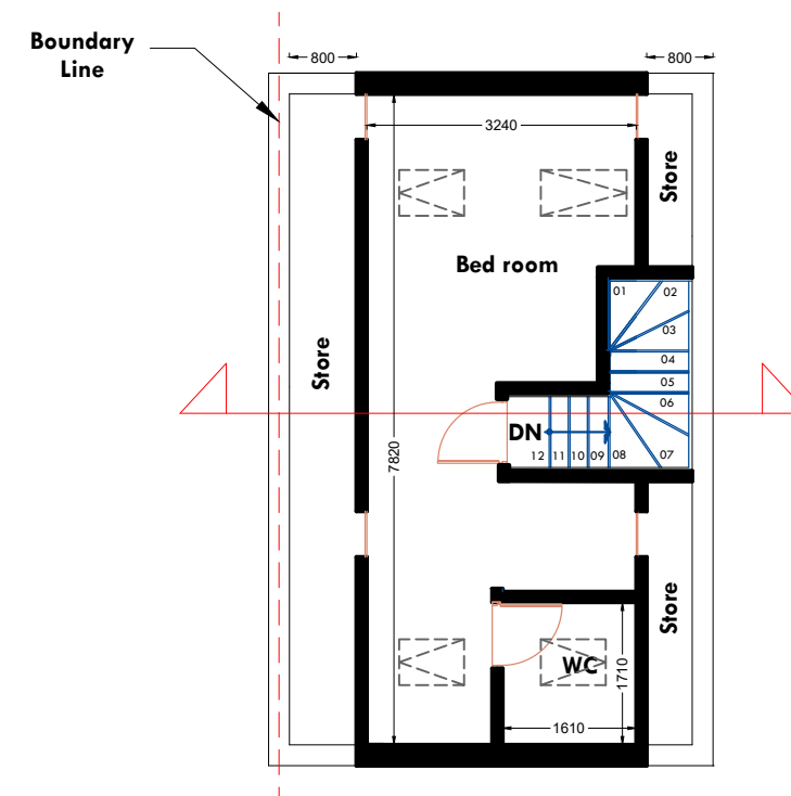
PROPOSED LOFT PLAN
