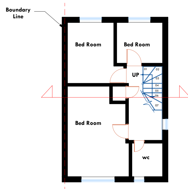
PROPOSED 1ST FLOOR PLAN
