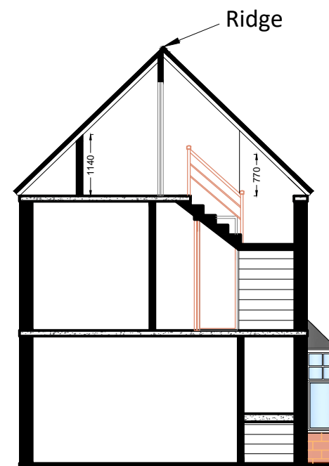
PROPOSED LOFT SECTION
