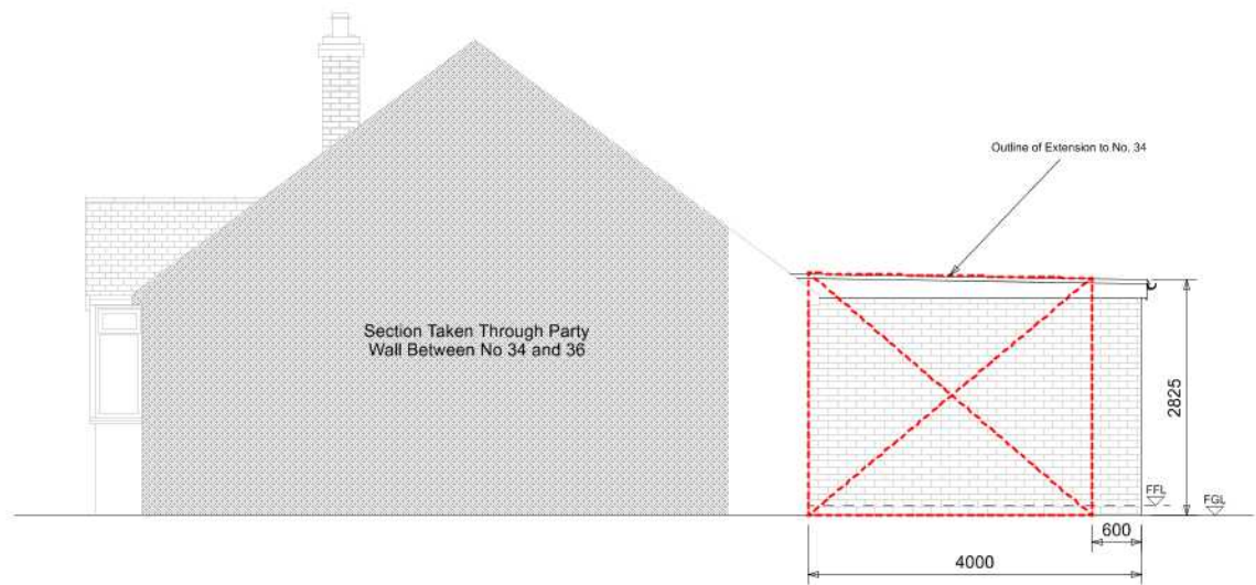
Proposed Side Elevation Viewed from No. 34
