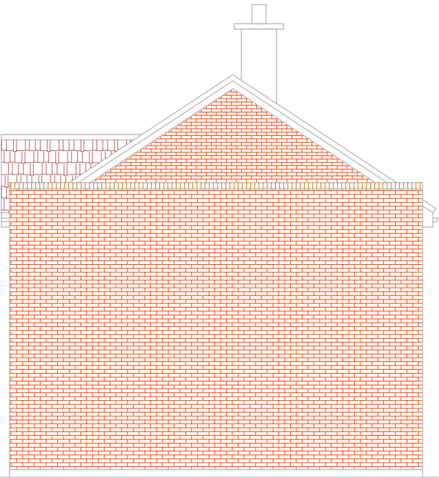
EXISTING SIDE ELEVATION -1
