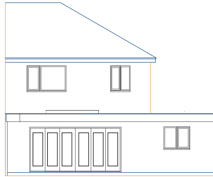
Rear Elevation
