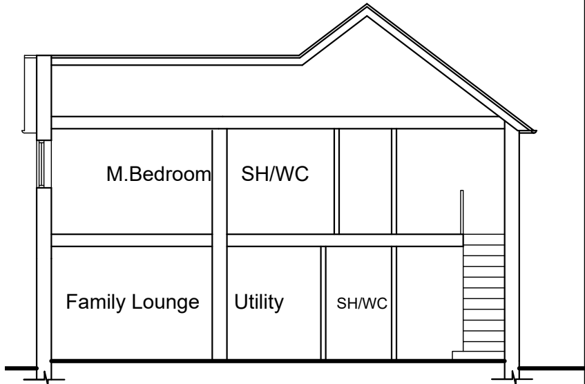
Proposed Section AA
