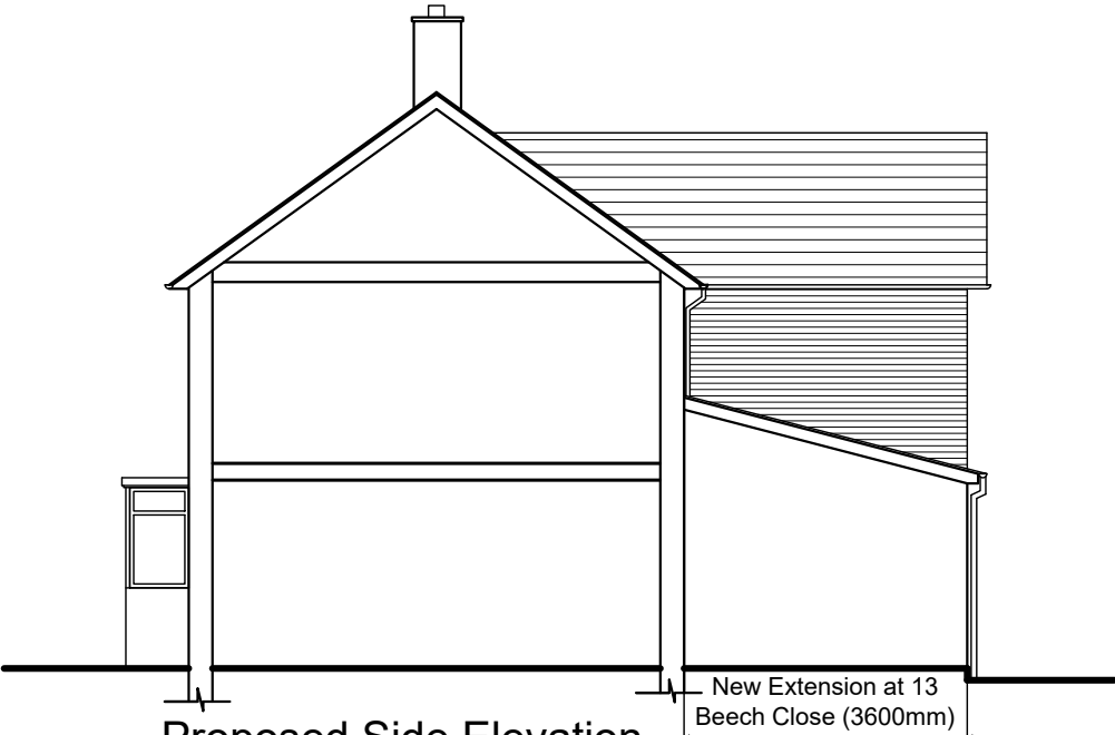
Proposed Side Elevation (No: 15 Beech Close shown in section)
