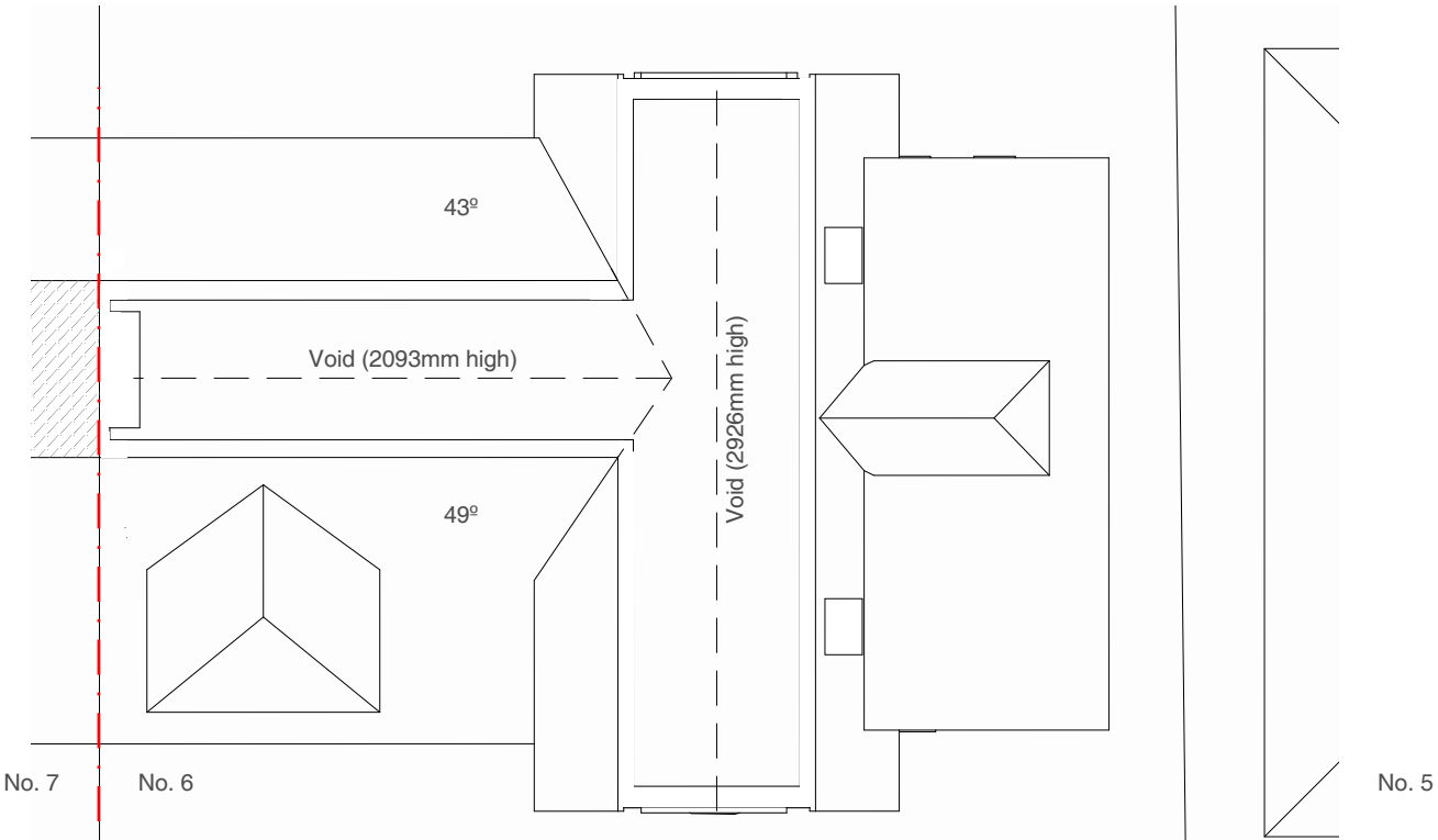
Existing Loft Floor Plan
