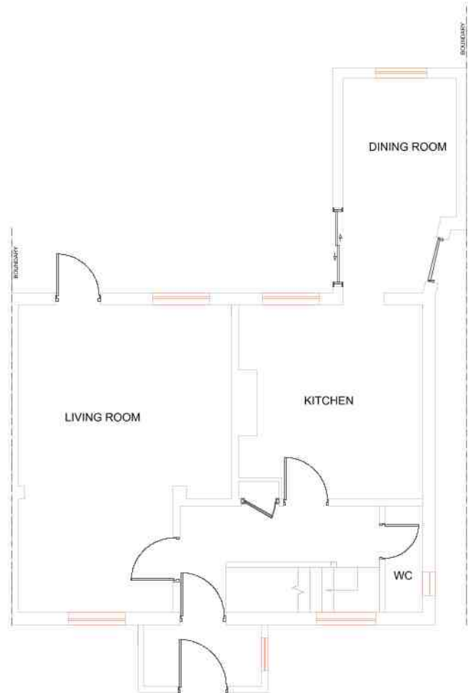
EXISTING GF PLAN
