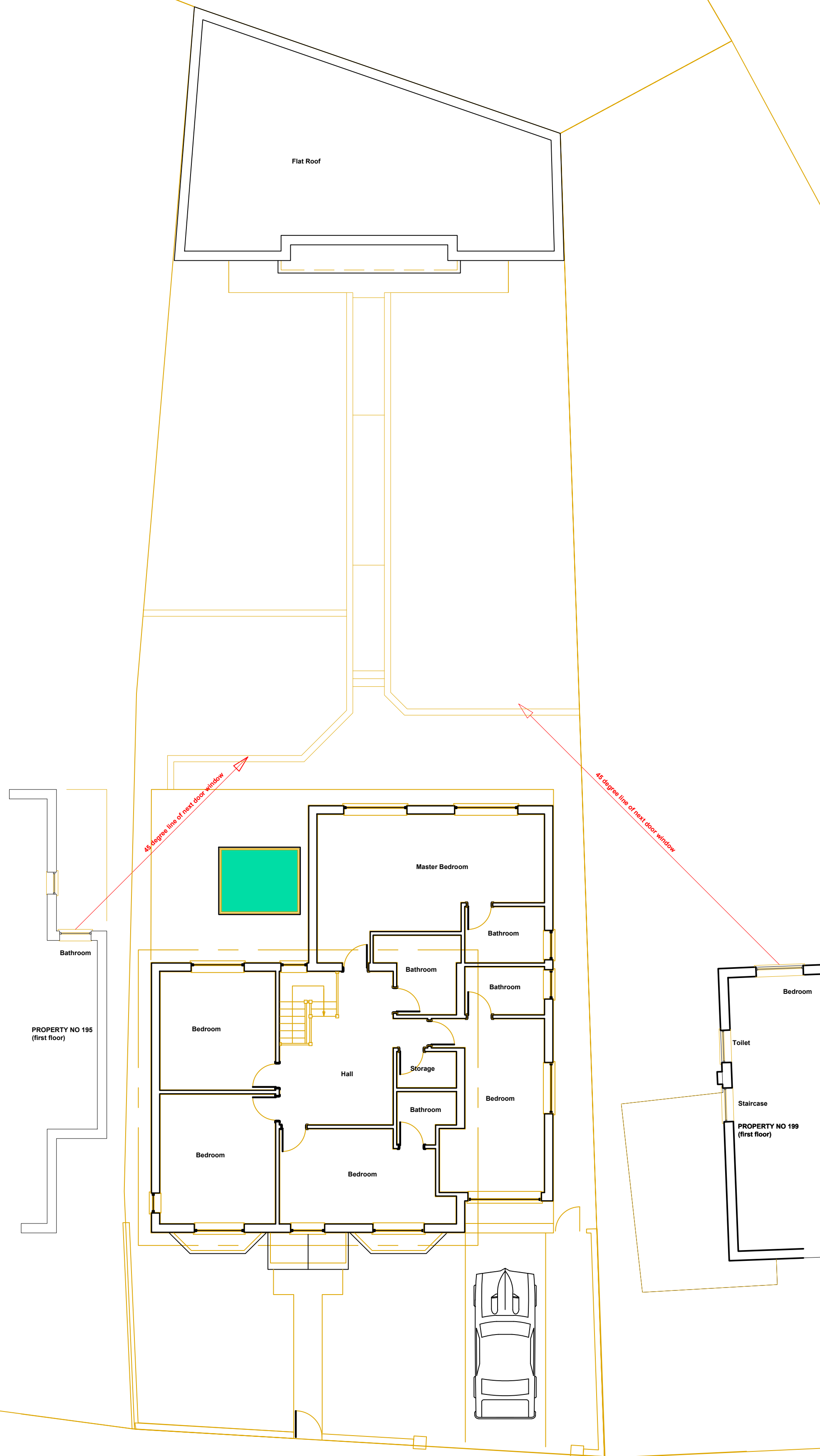
EXIST FIRST FLOOR PLAN
