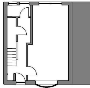
Proposed ground floor plan 1:100
