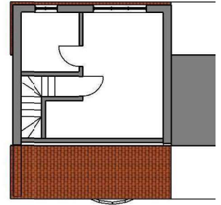
Proposed loft plan 1:100
