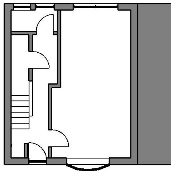
Proposed ground floor plan 1:100
