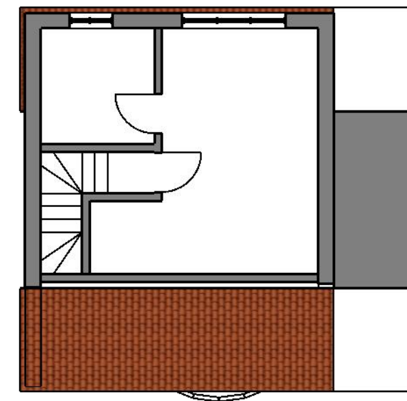
Proposed loft plan 1:100
