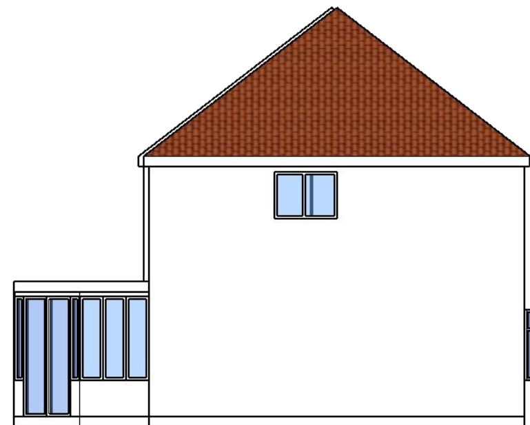
Existing left elevation 1:100
