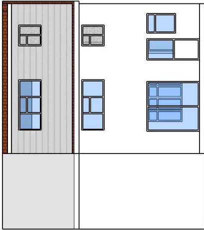
Proposed rear elevation 1:100
