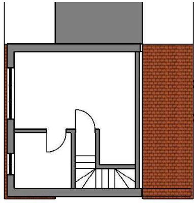
Proposed loft plan 1:100
