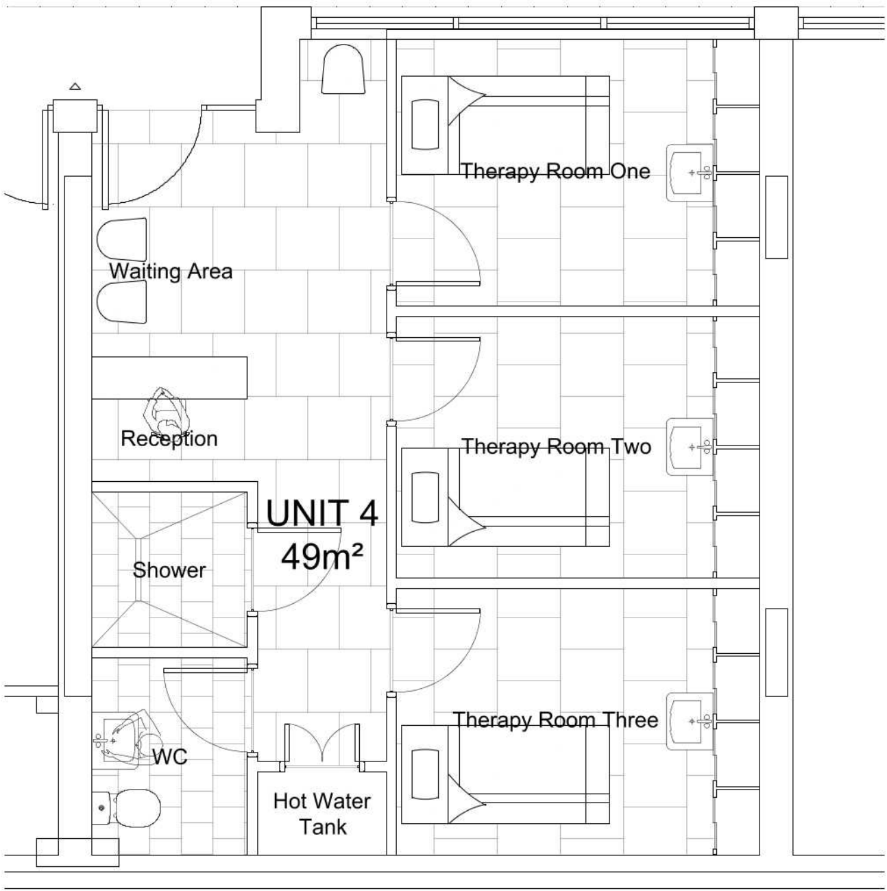
PROPOSED FLOOR PLAN A2 Sheet | Scale 1 : 50
