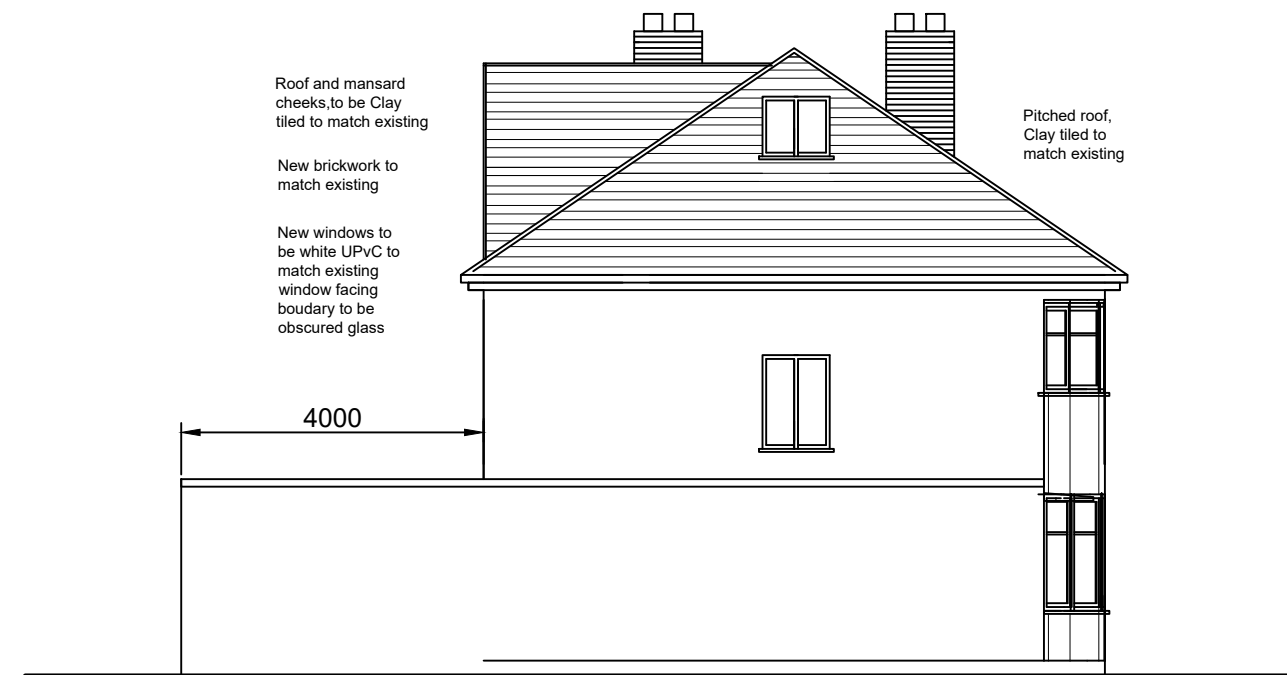
PROPOSED SIDE ELEVATION (DETACHED END)
