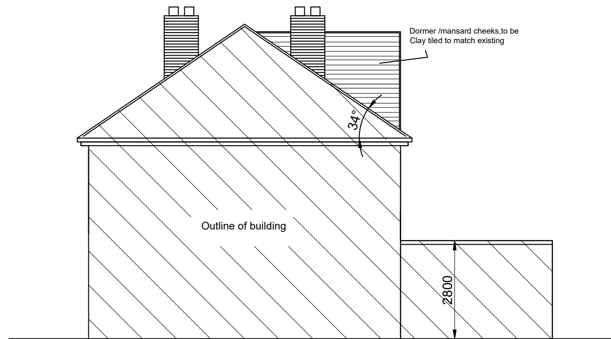
PROPOSED SIDE ELEVATION (ADJACENT TO NO.9)
