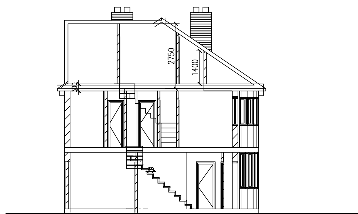
PROPOSED CROSS SECTION
