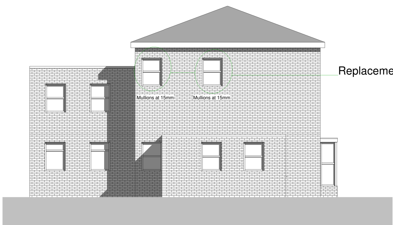
West elevation - Proposed 1 : 100
